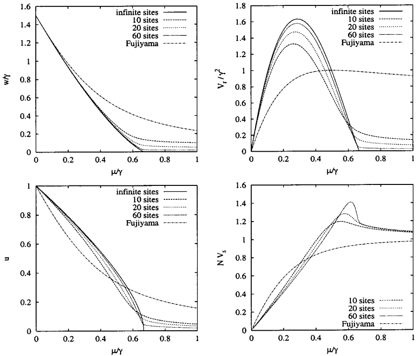
Fig. 6. Equilibrium behavior of fitness and surplus of the symmetric fitness model with finite sequence length. Results for the Fujiyama model with scaling \alpha = \gamma/2 are also shown.
