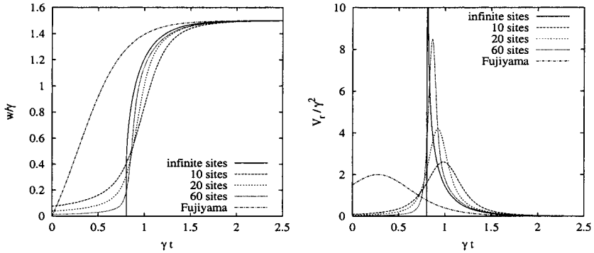
Fig. 8. Time evolution of the equidistribution of genotypes in the zero mutation-limit of the symmetric fitness model for different sequence lengths.
