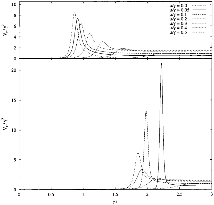
Fig. 9. Time evolution of the variance of the fitness in the symmetric fitness model with sequence length N=60 . Results are shown for varying mutation rates and two different starting configurations.
