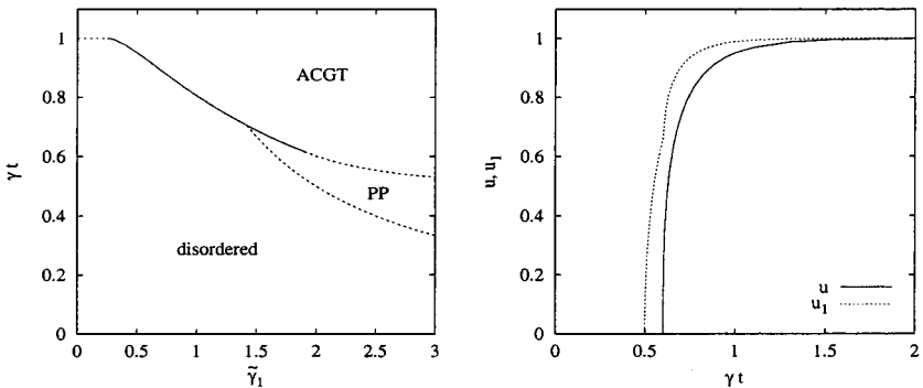
Fig. 7. Dynamical phase diagram of the transition–transversion model for vanishing mutation starting from the equidistribution. (Solid: first order; dashed: second order transition). Right: Time evolution of the surplus components for \tilde{\gamma}_1 = 2 .
