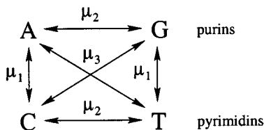
Fig. 1. Molecular mutation scheme according to the Kimura 3 ST model.
