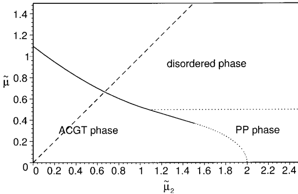
Fig. 4. Phase diagram of the transition–transversion model with symmetric fitness landscape and Kimura 2 parameter mutation scheme. Solid and dotted lines correspond to first and second order phase transitions respectively. The dashed line indicates the Jukes–Cantor mutation scheme.
