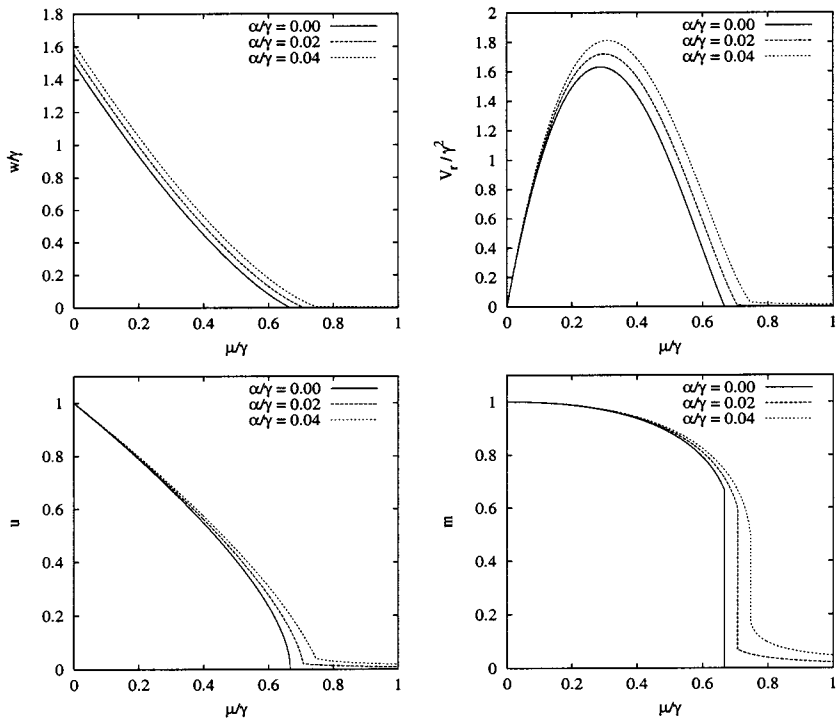
Fig. 3. Mean fitness and its variance, surplus and magnetization in the symmetric fitness model for various linear parts of the fitness function in the infinite sites limit.
