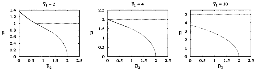
Fig. 5. Phase diagrams for anisotropic fitness landscapes \gamma_1 > \gamma_2 = \gamma_3 \equiv \gamma and Kimura 2 parameter mutation scheme. Solid and dotted lines correspond to first and second order phase transitions, respectively.
