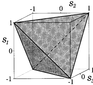
Fig. 2. Permutation invariant configuration space of the four-state model in surplus coordinates.
